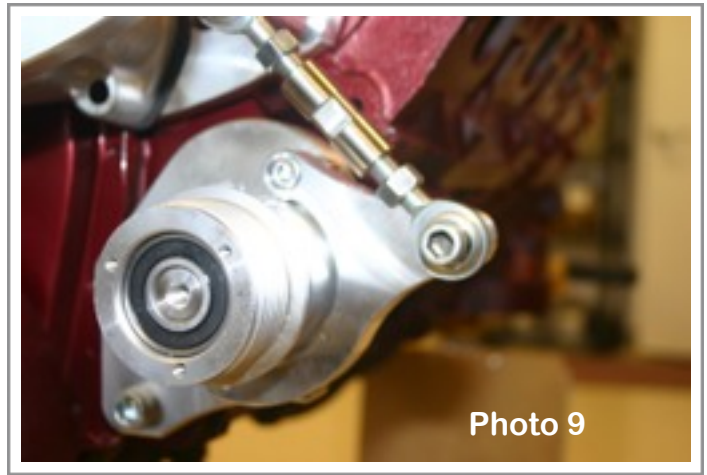
21178-C mounts over the top of the 30606-A bracket as shown
